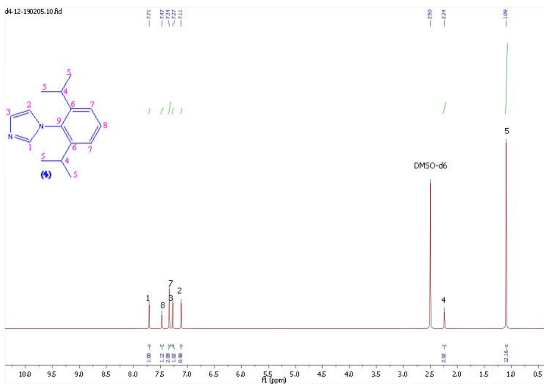
Figure 7. Spectre RMN ^1\text{H} de 2,6-diisopropylaniline (4) en DMSO- \text{d}_6
