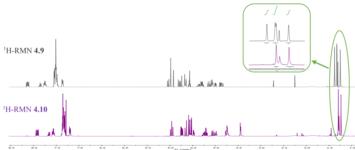
Figure 4.6 : Spectres ^1\text{H} -RMN des pseudo-disaccharides 4.9 et 4.10 .
