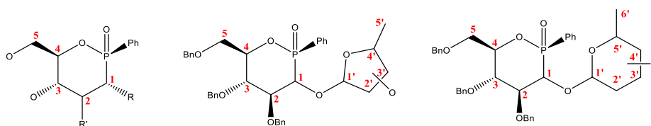
NMR numberings of phostines and pseudo-disaccharides
