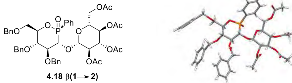
Figure 4.8 : Structure cristallographique de pseudo-disaccharide 4.18 \beta(1 \rightarrow 2) .
