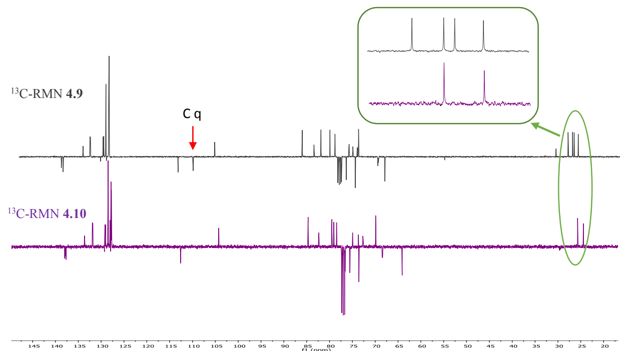
Figure 4.7 : Spectres ^{13}\text{C} -RMN des pseudo-disaccharides 4.9 et 4.10 .
