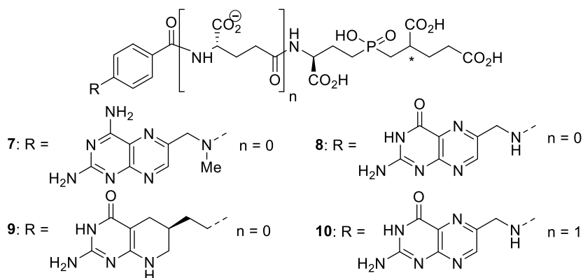
Figure 1.8 : Modification structurale des analogues phosphinates.
