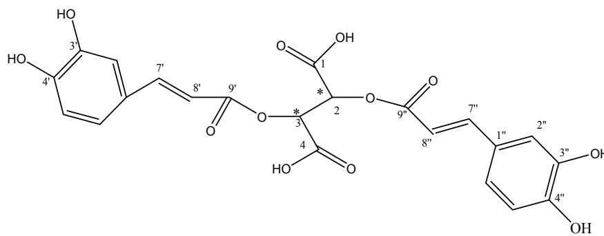
Acide di-E-caffeoyl-(2S,3S)-tartarique (acide chicorique)
