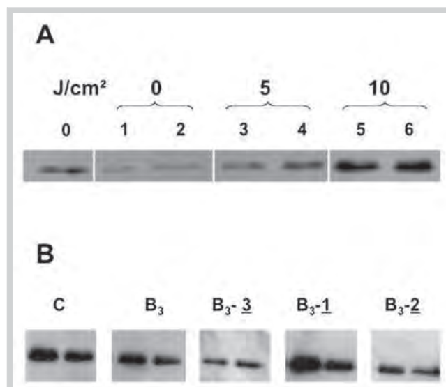
Fig. 5 Inhibition of UVA-mediated MMP-3 expression (Western blotting) in human skin fibroblasts (49 yrs old individual) by caffeic acid derivatives. UVA irradiation (human skin fibroblasts at confluency were used at passage 5): A influence of increasing dose of UVA (0, 5, and 10 J/cm 2 ) on MMP-3 expression; B cells were incubated with B 3 , (+)-chicoric acid (1), chicoric acid monomethyl ester (2), or caffeic acid (3) (1 \mu g/mL) before UVA exposure (10 J/cm 2 ). This figure is representative of three distinct experiments.
