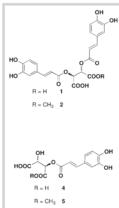
Fig. 1 Chemical structures of compounds isolated from propolis.
