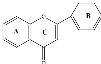
Figure-9 : Phenyl-2- chromone.
