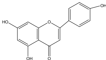
5, 7, 4'-trihydroxyflavone (apigénine).
