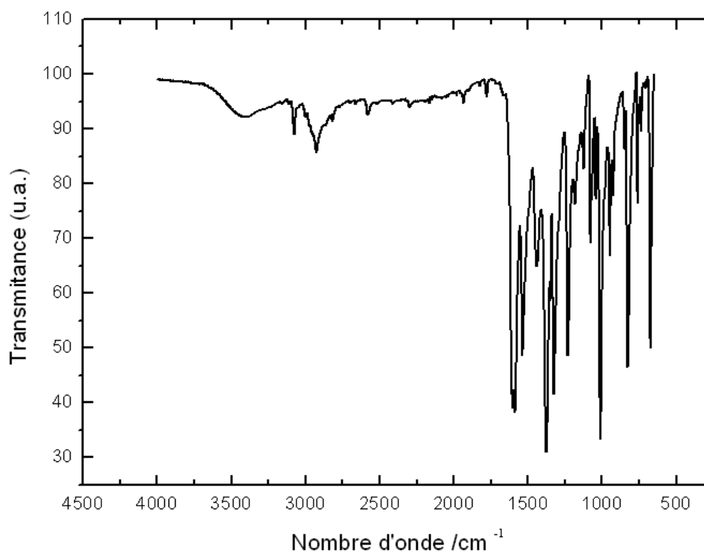
Figure 1 : Spectre infra rouge du composé [\text{Cu}(\text{C}_2\text{H}_3\text{O}_2)_2(\text{C}_7\text{H}_{10}\text{N}_2)_2]
