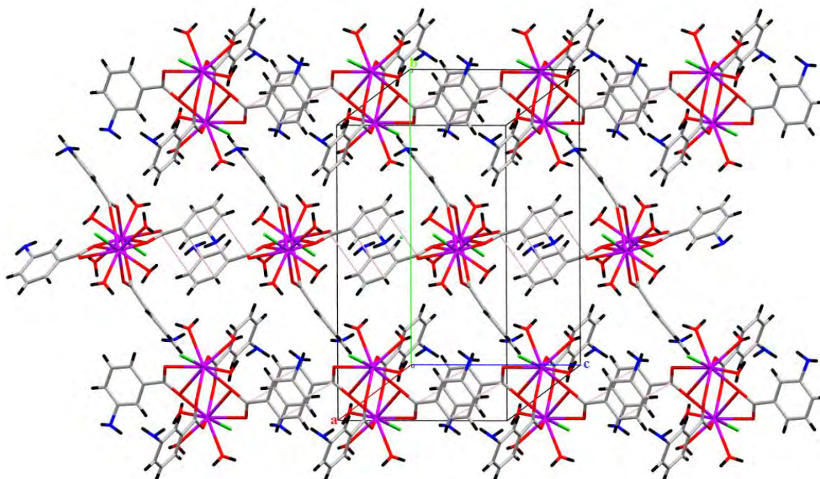
Figure 14: Interactions de type \pi - \pi .
