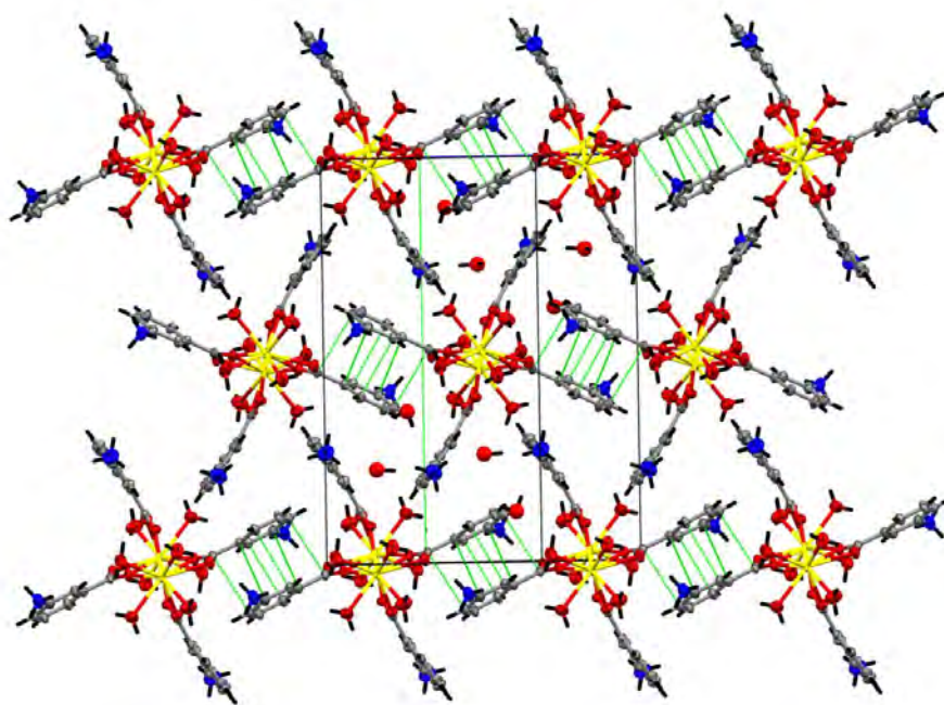
Figure 10: Les interactions de type \pi - \pi
