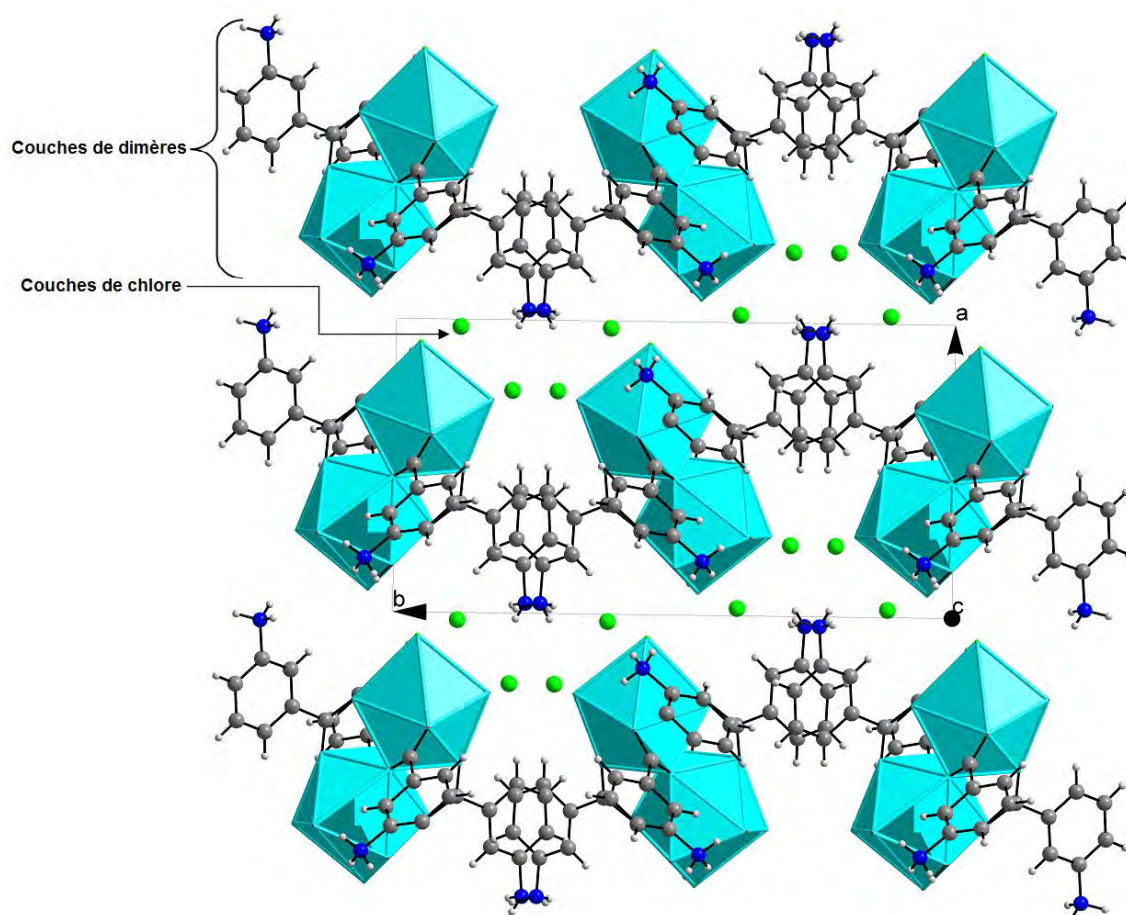
Figure 7: Projection de la structure selon le plan (a b)
