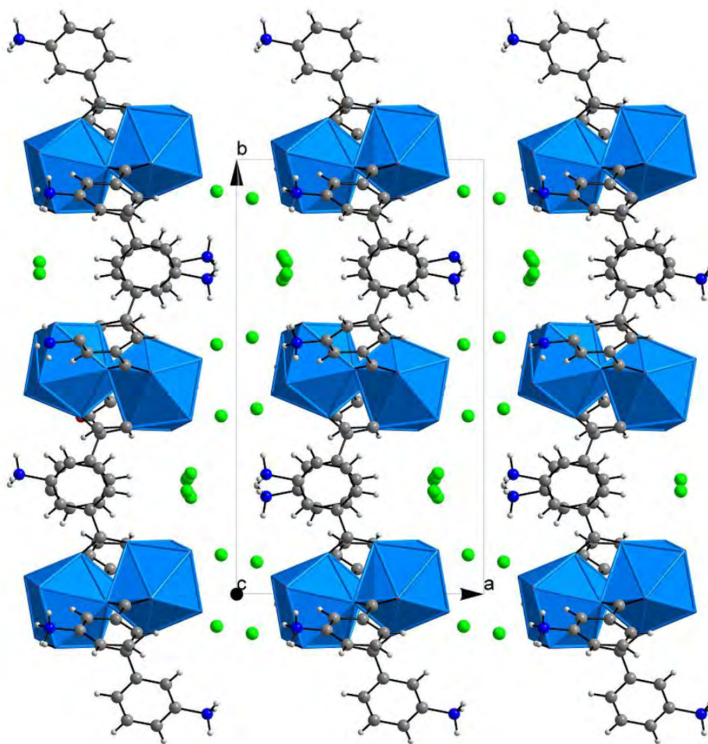
Figure 5: Projection de la structure selon le plan (a b)
