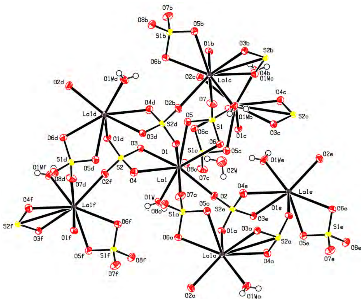
Figure 1 : La structure du composé [\text{La}_2(\text{SO}_4)_3(\text{H}_2\text{O})_2] \cdot 2\text{H}_2\text{O} (a): 1-x, -1/2+y, 1/2-z , (b): 1-x, 1/2+y, 1/2-z , (c): -x, 1-y, -z , (d): 1-x, 1-y, 1-z , (e): x, 1/2-y, -1/2+z , (f): x, 1/2-y, 1/2+z
