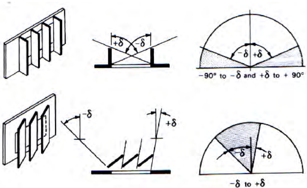
Figure 4- 30 : Type de protection verticale. Source: S V SZOKOLAY, 1979.
