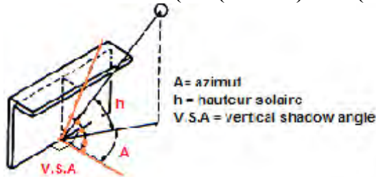
Figure 4- 18: Vertical shadow angle (VSA). Source: S. SOCKOLAY, 1979.
