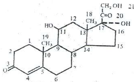
Figure 1 - Structure du cortisol
