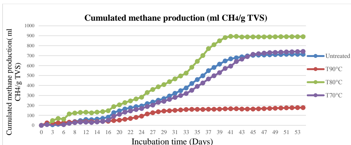
Figure 2. Effect of thermal pretreatments on biomethane production from TWW.
