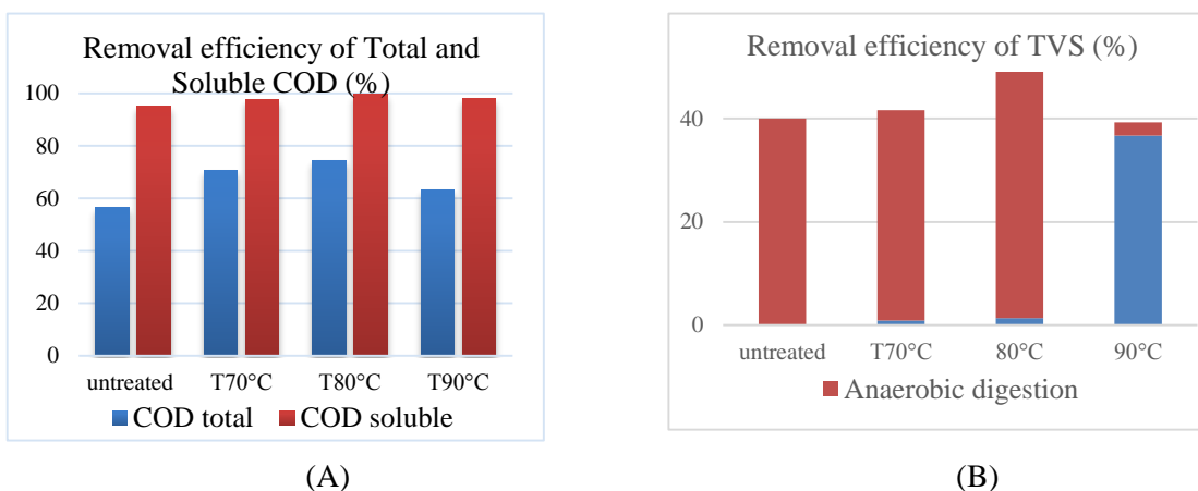
Figure 3. Removal efficiency of total and soluble COD (A) and TVS (B)
