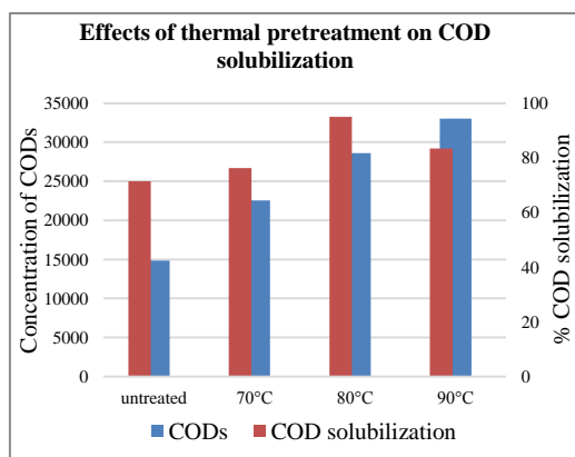
Figure1. Effects of thermal pretreatment on COD solubilization
